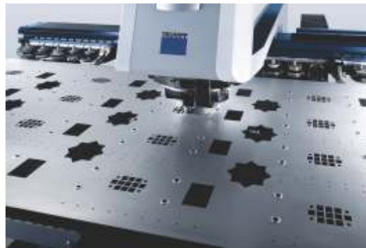
Trumpf trupunch 3000 S11 Turret punching Machine
