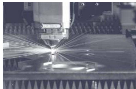
AMADA LCG Laser cutting Machine
